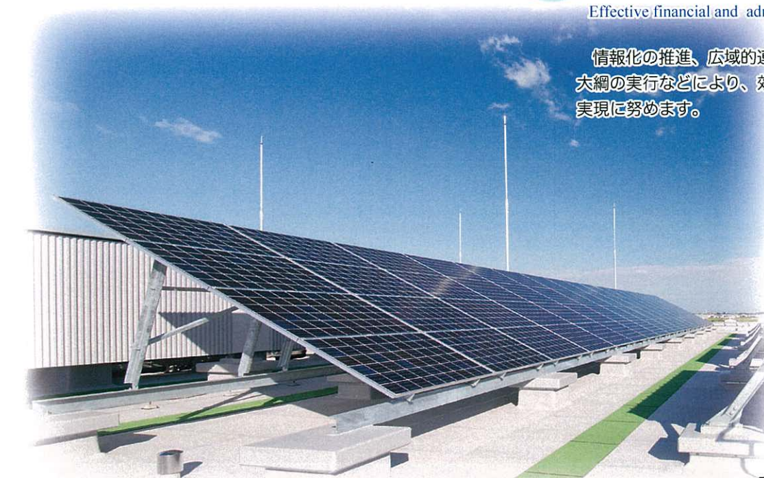
庁舎の太陽光発電パネル Solar power panel of the government facilities
